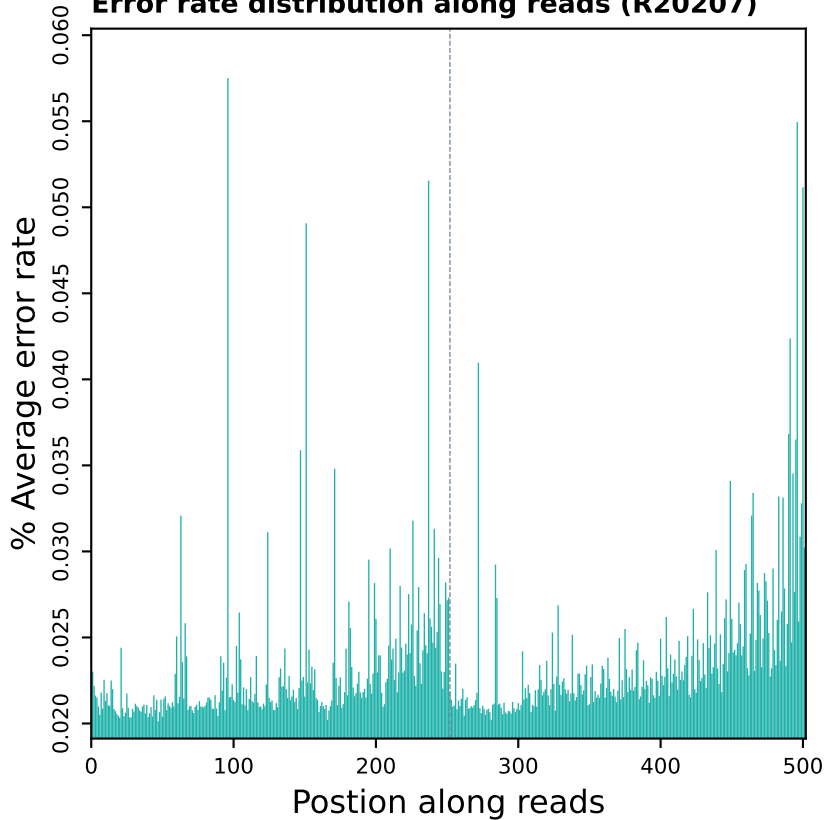
Error rate distribution along reads (R20207)
